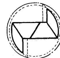
Fig. 2 Shows the same cutter after several regrinds with no clearance.
