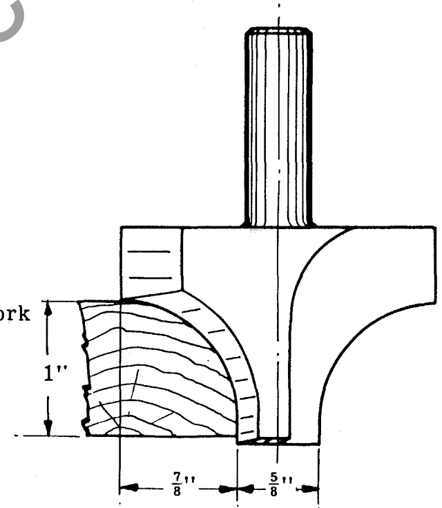
Maximum dimension of moulding on Router.
