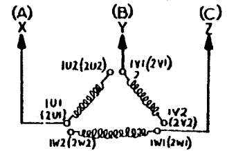
DRIVE MOTOR & EXCITATION WINDINGS 50HZ
